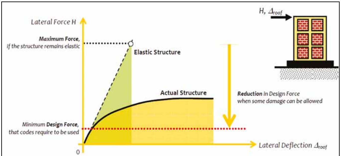
Figure 3 [4] : Basic strategy of earthquake design: Calculate maximum elastic forces and reduce by a factor to obtain design forces
