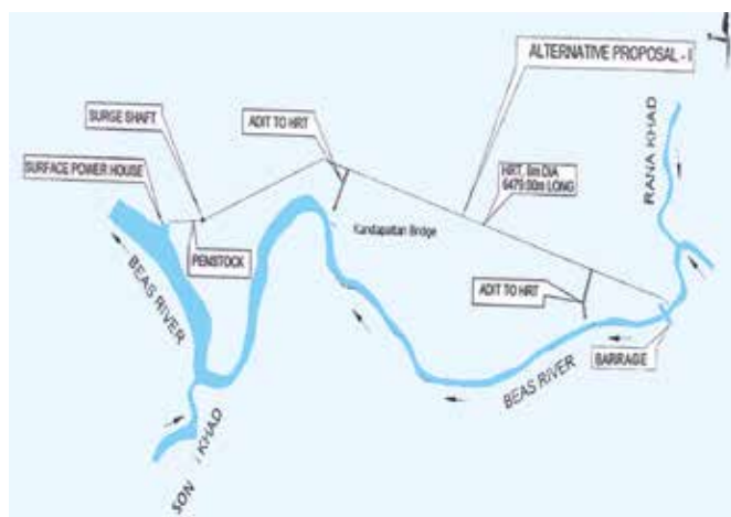
Figure-1 Typical Run-Off the River Hydel Project in Beas River
