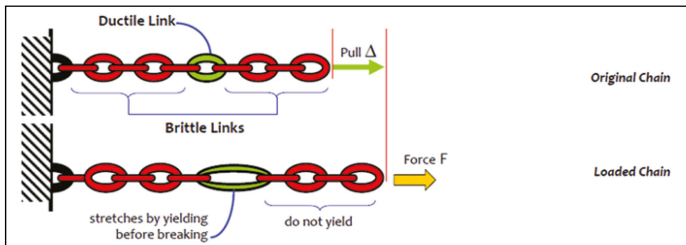
Figure 5 [4] : Ductile chain
